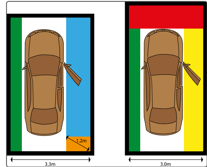
Figure 3.2.7 Garage design measurements (assumes no passengers)
