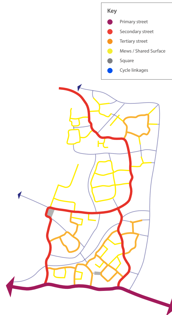
Figure 3.3.8 Hierarchy of movement, Loves Farm
